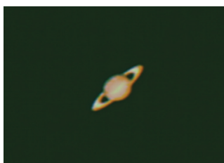
Saturn
